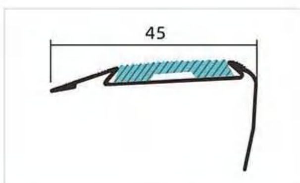
Floor strip A | 直角地板压条
